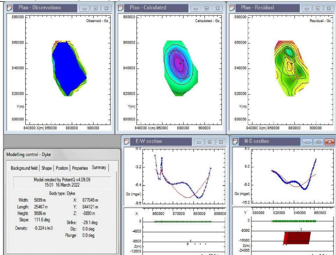
Fig 13: Result of model point K5 using a dyke model
